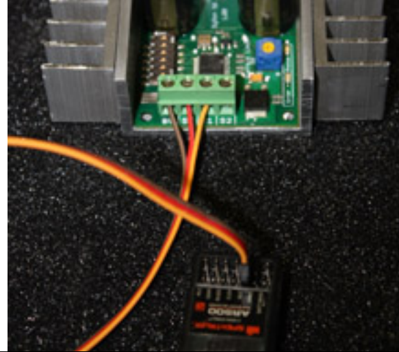
Figure 5.1: R/C connection
