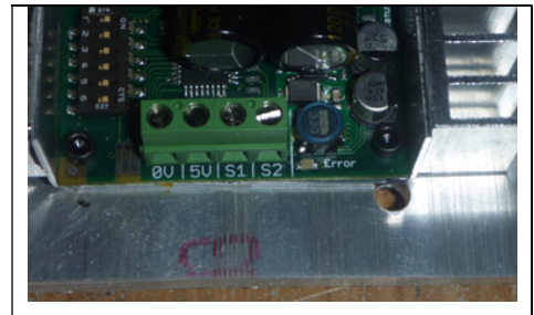
Figure 2.4: Mounted directly to a metal frame
