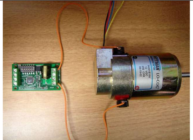
The motor connects to terminals M1 and M2
