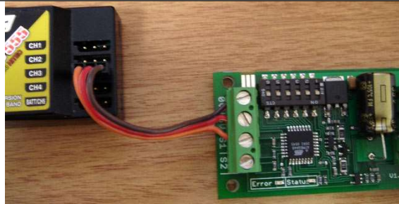
Figure 5.1: R/C connection
