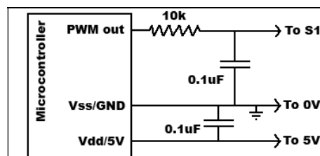
Figure 4.1: Fast filtering
