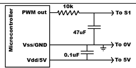
Figure 4.2: Very smooth filtering
