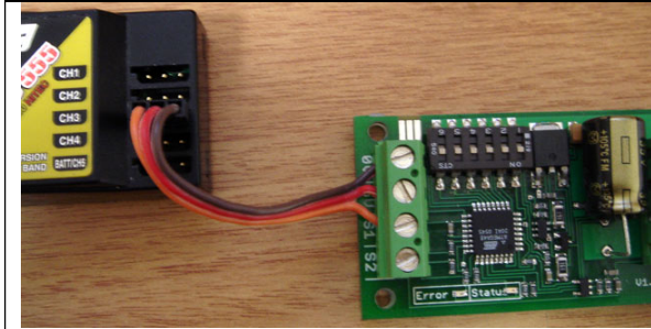
Figure 5.1: R/C connection
