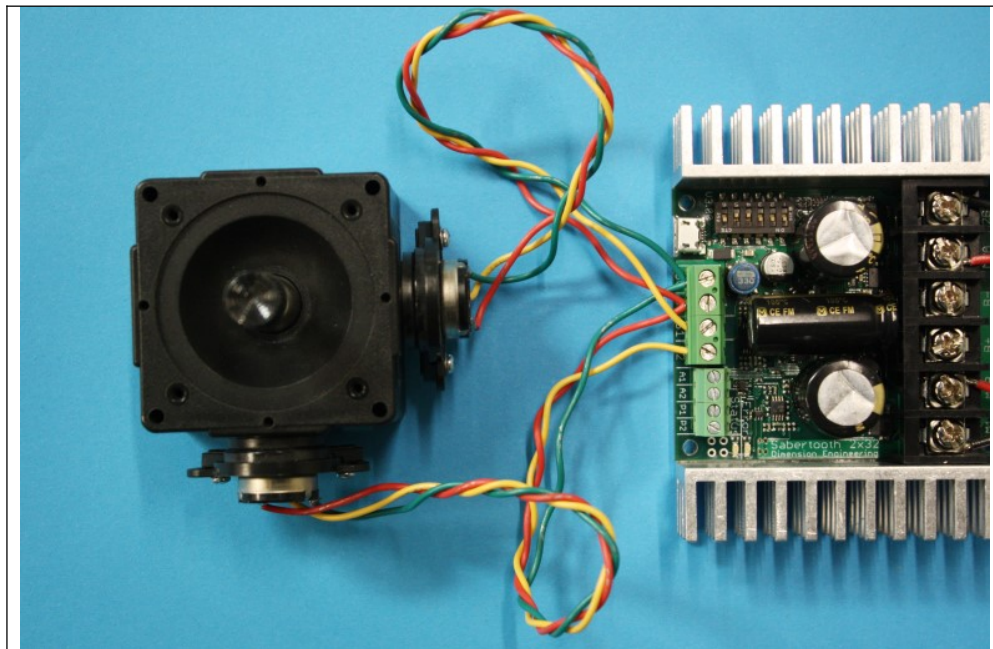
An analog joystick connected to a Sabertooth 2x32
