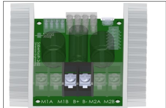
The main power inputs are labeled B+ and B-
