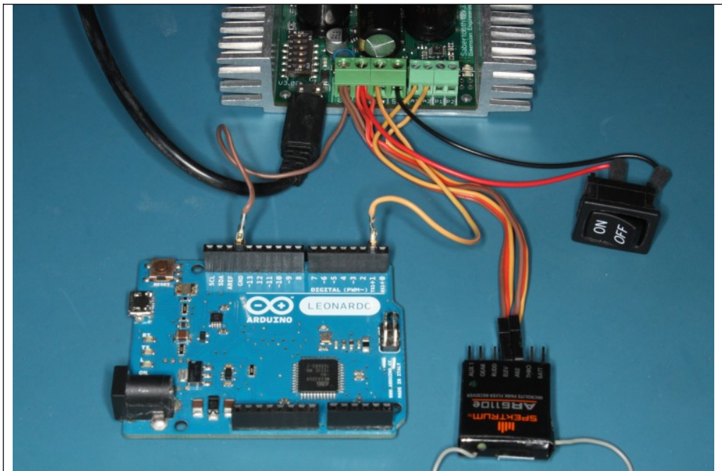
A Sabertooth 2x32 connected to a serial input and a radio receiver, with a switch to select the controlling device and USB monitoring.
