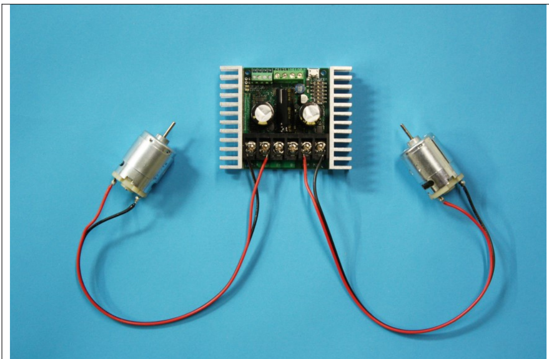
Two small motors connected to the Sabertooth 2x32's Motor Outputs.
